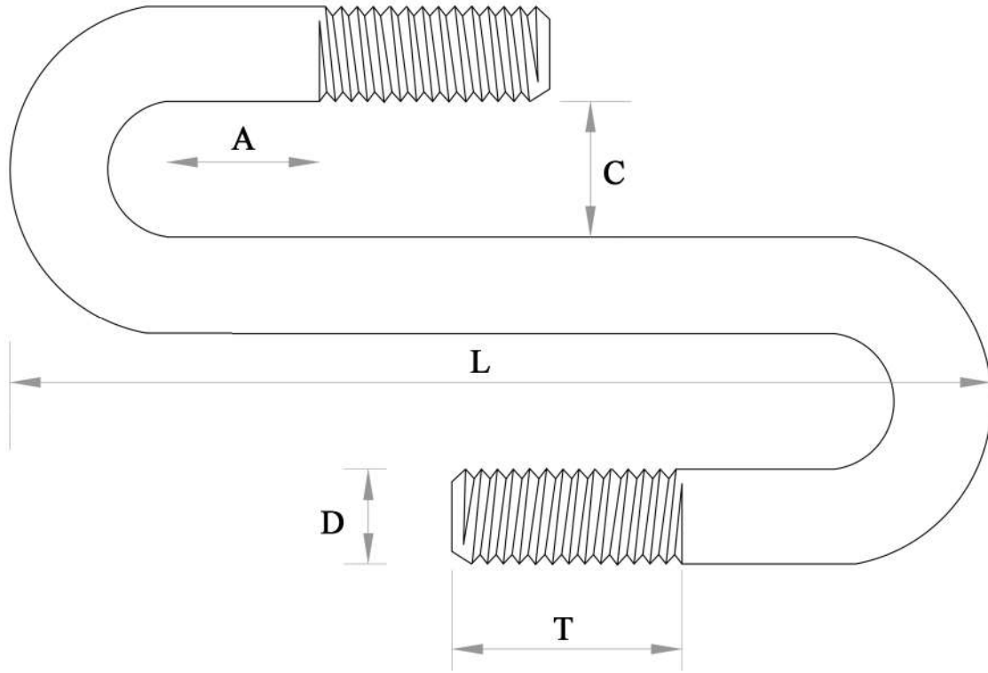
S - HOOK BOLT
