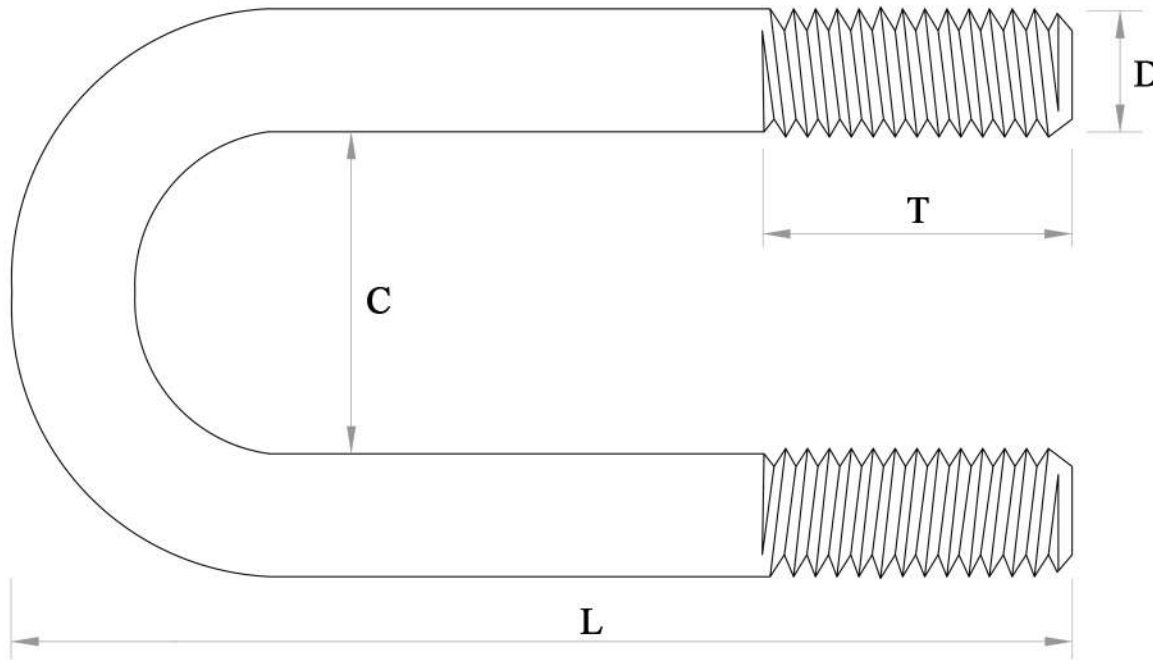
ROUND U - BOLT
